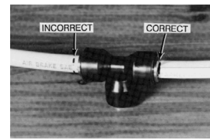
3 – Install Tube into the Fitting
