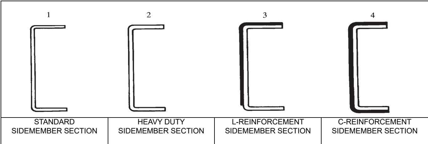
Figure 2.1 Frame Rails and Reinforcements (Typical) 01_0011
