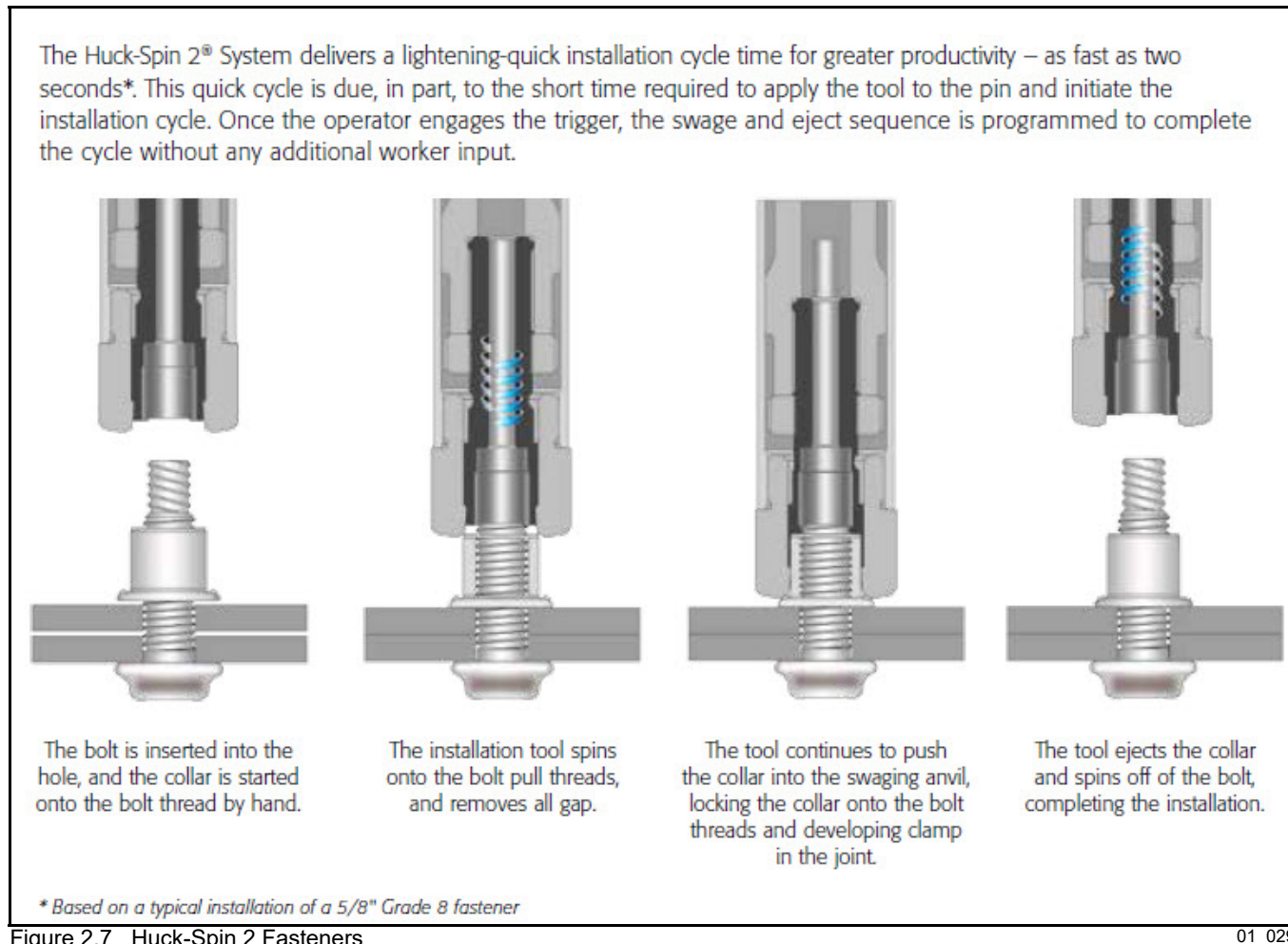
Figure 2.7 Huck-Spin 2 Fasteners
