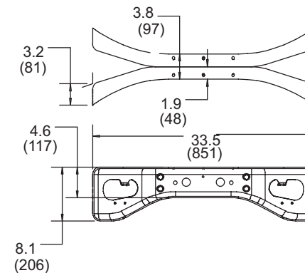
DOUBLE STAMPED CROSSMEMBER
