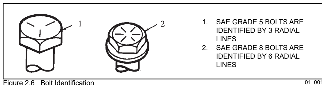
Figure 2.6 Bolt Identification
