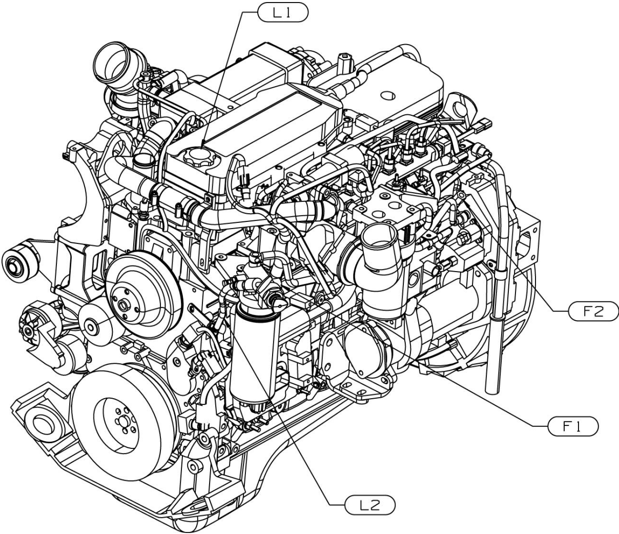
Cummins B6.7 Engine (Left Front)
