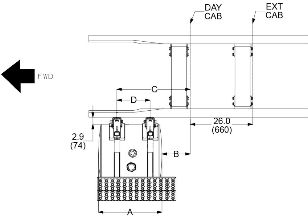
Single Round Fuel Tank with 2 Mounting Straps Mounted Left Side Under Cab (Top View)
