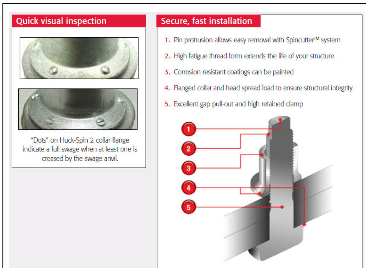
Figure 2.8 Huck-Spin 2 Installation
