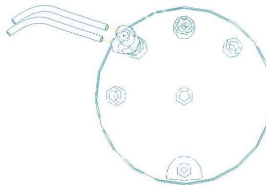
View displaying Pressure protection valve in end of Primary air tank with two supply tubes.
